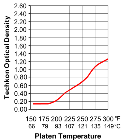
Static Sensitivity
